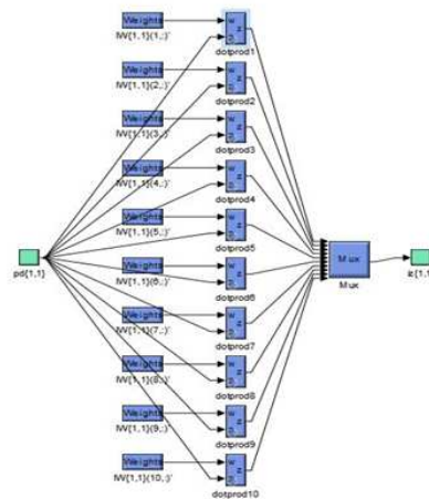
Figure 4: Hidden Layers of the Network
