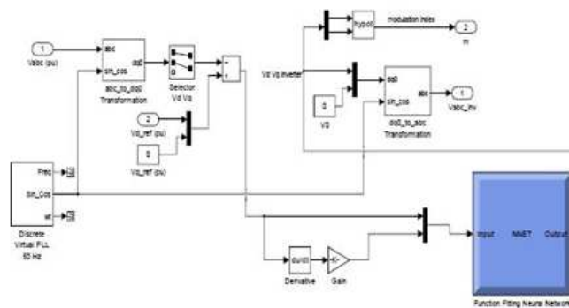
Figure 5: Artificial Neural Network Applied to 11 Level Cascaded H Bridge Multi Level Inverter
