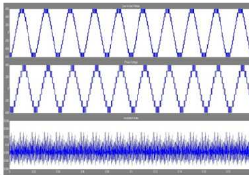
Figure 10: Line Voltage and Phase Voltage with Modulation Index Equal to 0.6
