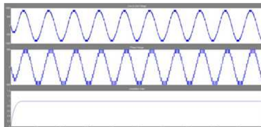
Figure 12: Line Voltage and Phase Voltage with Modulation Index Equal to 1 by Using PI Controller
