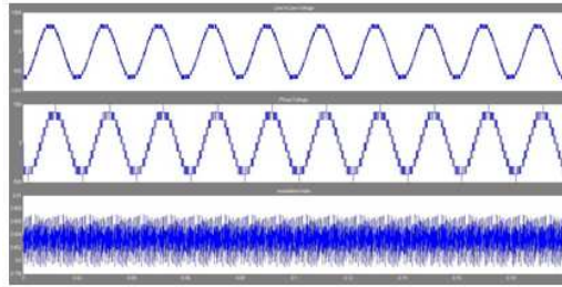
Figure 9: Line Voltage and Phase Voltage with Modulation Index Equal to 0.7
