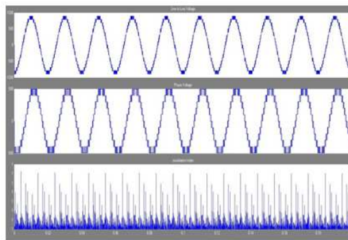
Figure 6: Line Voltage and Phase Voltage with Modulation Index Equal to 1
